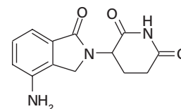
3-(4-amino-1-oxo-1,3-dihydro-2H-isoindol-2-yl) piperidine-2,6-dione
